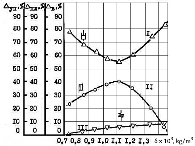
Figure 3 – The interchange of viscous (I), plastic (II) and elastic (III) properties of the molding sand during the compaction process
