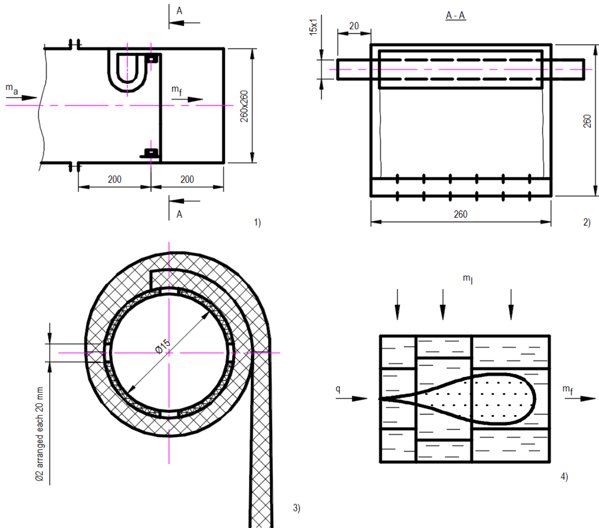
Figure 2 – Test facility for research of foam generation process: 1 – Foam generator; 2 – spray device; 3 – connection of capillary porous structure; 4 – bubble dynamics in structure
