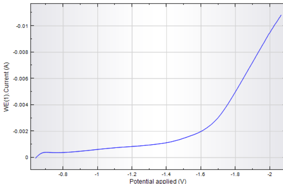
Figure 2 – Cathode potentiodynamic polarization curve of the thallium electrode in the sodium nitrate solution: [\text{NaNO}_3] = 100 \text{ g/l} ; v = 50 \text{ mV/s} ; t = 25 \text{ }^\circ\text{C}
